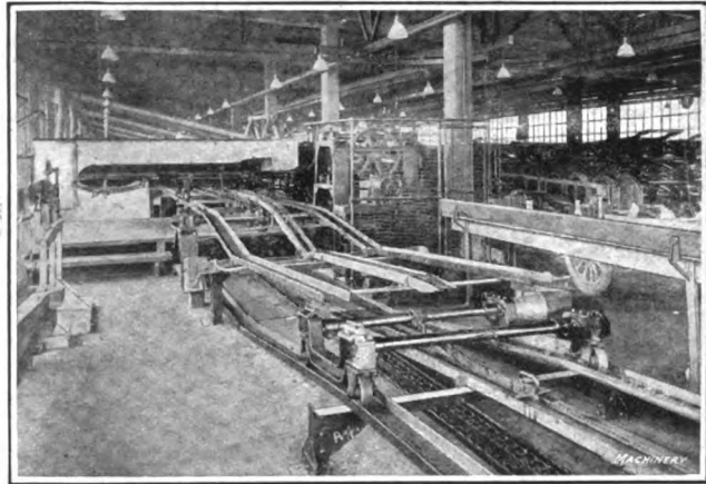
Fig. 19—Here we show a conveyor system installed by Palmer-Bee Co., of Detroit, Mich., for handling automobile frames in Paige-Detroit Motor Car Co.'s plant. Empty trucks return through tunnel and are caught by a hook on the conveyor. They run back over hinged section of track and receive frames from trolley system. One truck is coming up the incline and another is on upper level of track with a frame on it.
